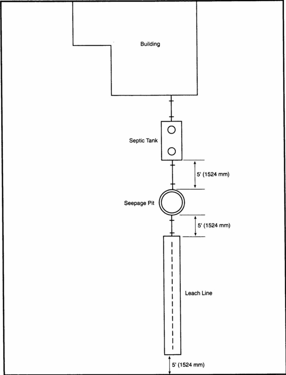
Figure K-4 Septic Tank System with a Combination Seepage Pit and Leach Line
